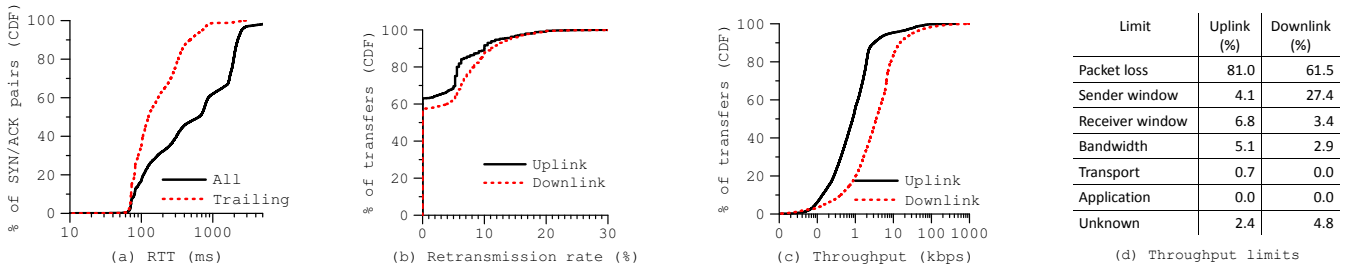
Figure 6: Performance of TCP transfers in Dataset1.
